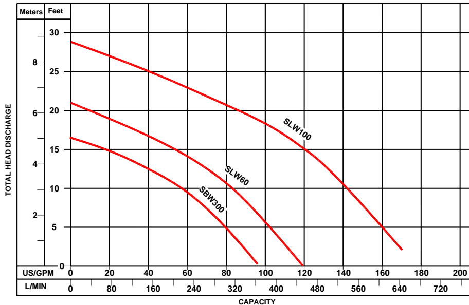
PUMPING CURVES SBW / SLW SERIES
